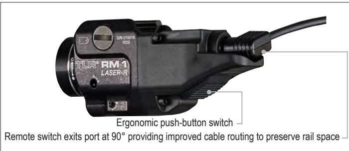
Mode selector toggle switch for Laser only, Light only or Light/Laser combo modes
