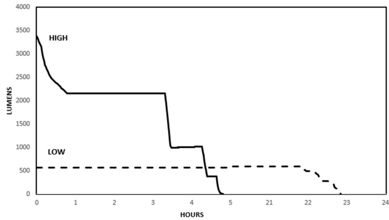
PERFORMANCE CURVE
