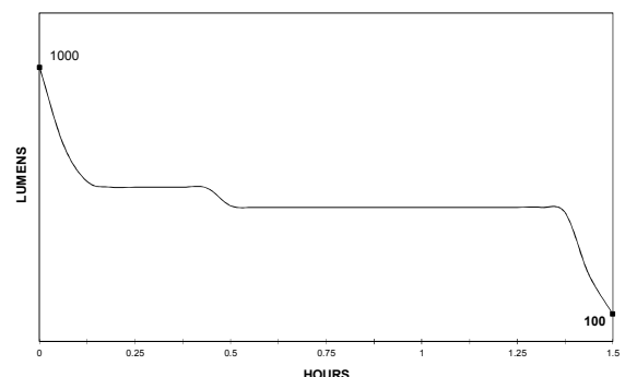
PERFORMANCE CURVE
