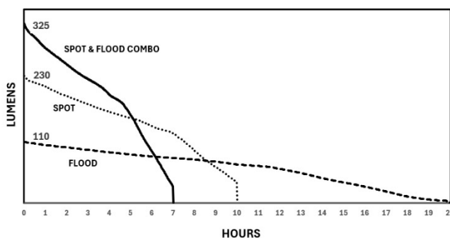
PERFORMANCE CURVE
