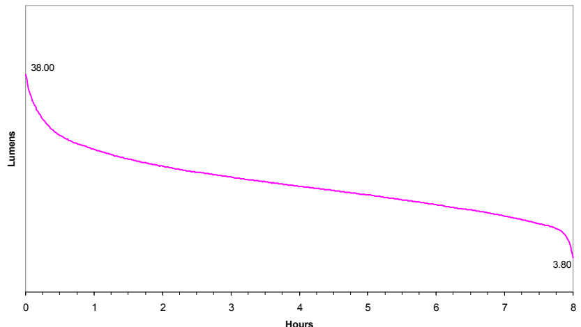
PERFORMANCE CURVE
