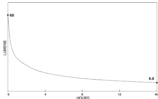
2AAA PROPOLYMER HAZ-LO PERFORMANCE CURVE
