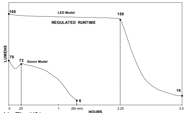
PERFORMANCE CURVES
